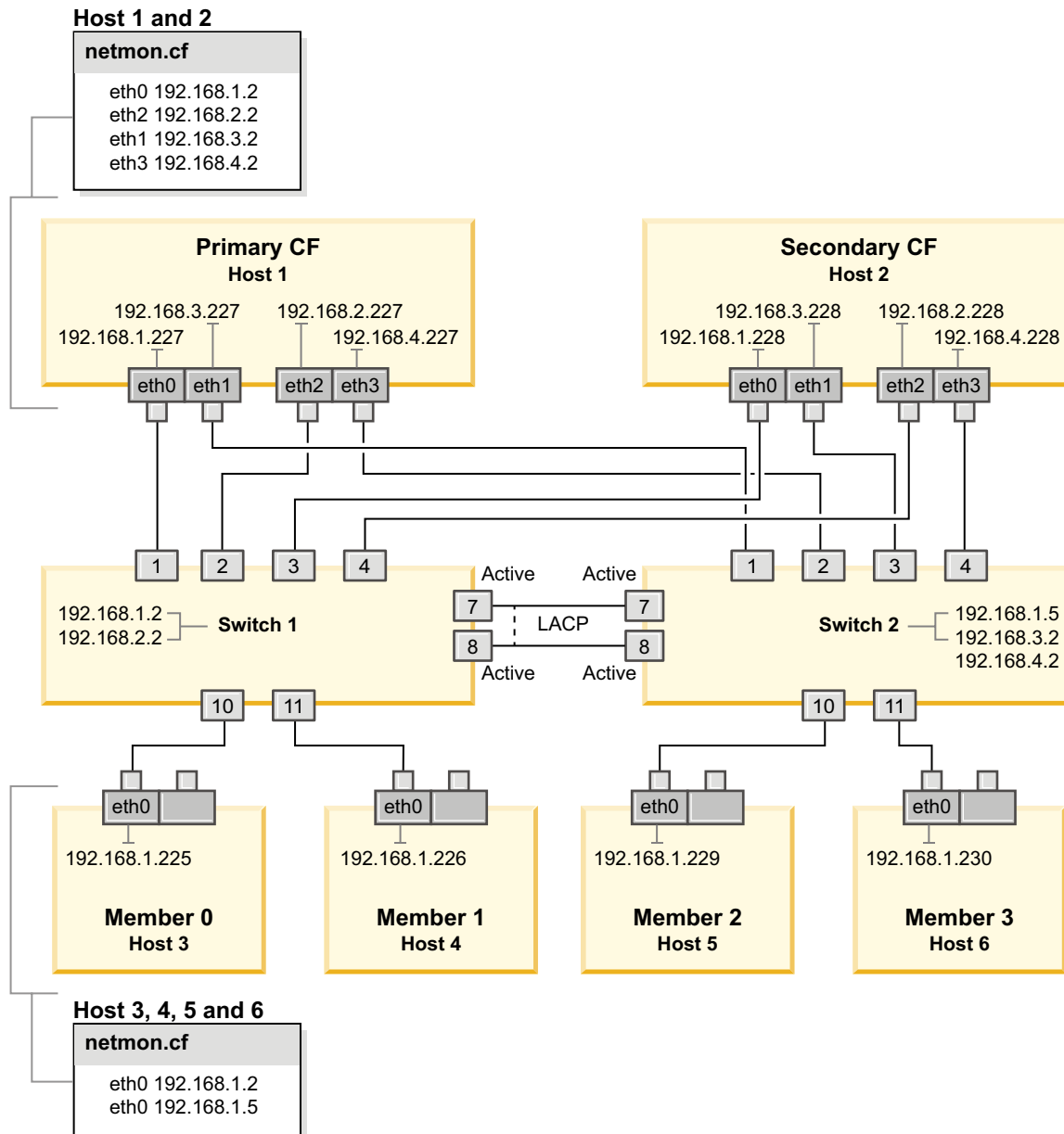
Figure 21. Two CFs and four members connect to two switches.
