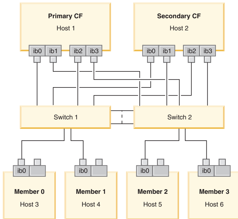
Figure 18. The 2 CFs and four members connect to two switches.
