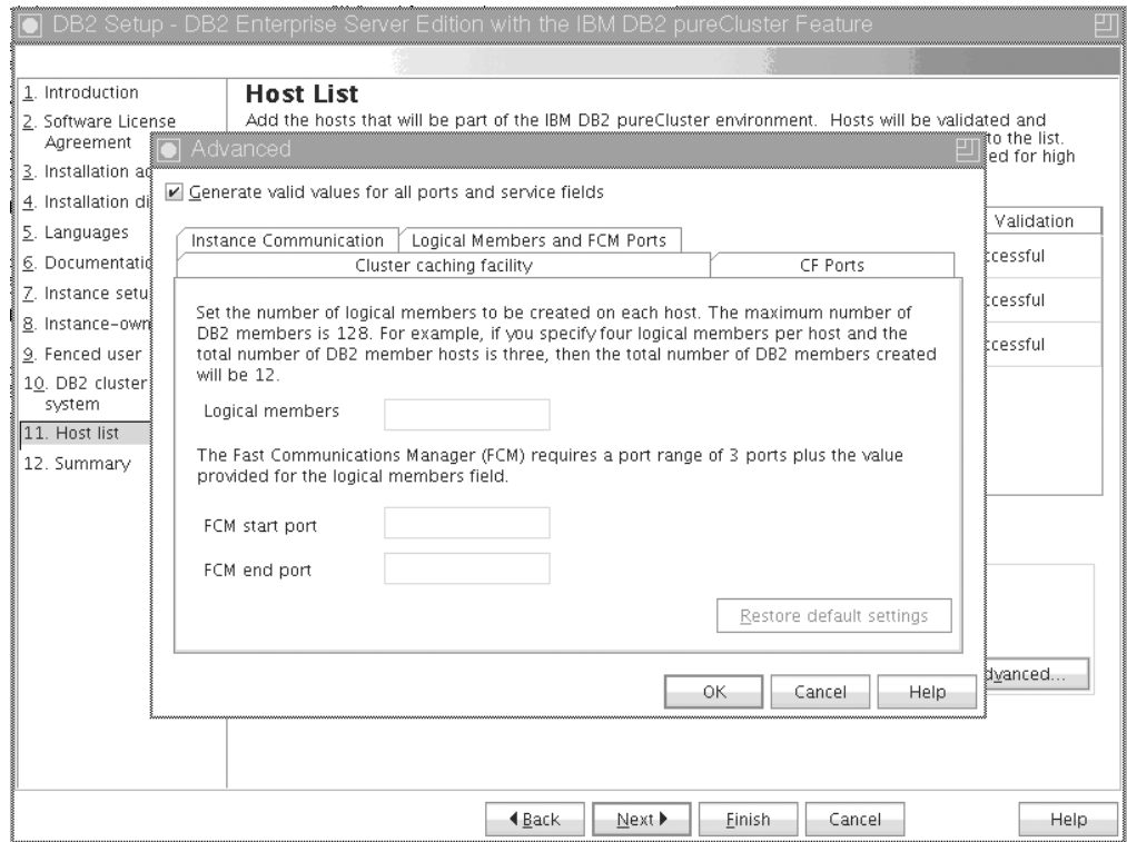
Figure 43. Advanced Instance Settings - Logical members and FCM Ports tab
