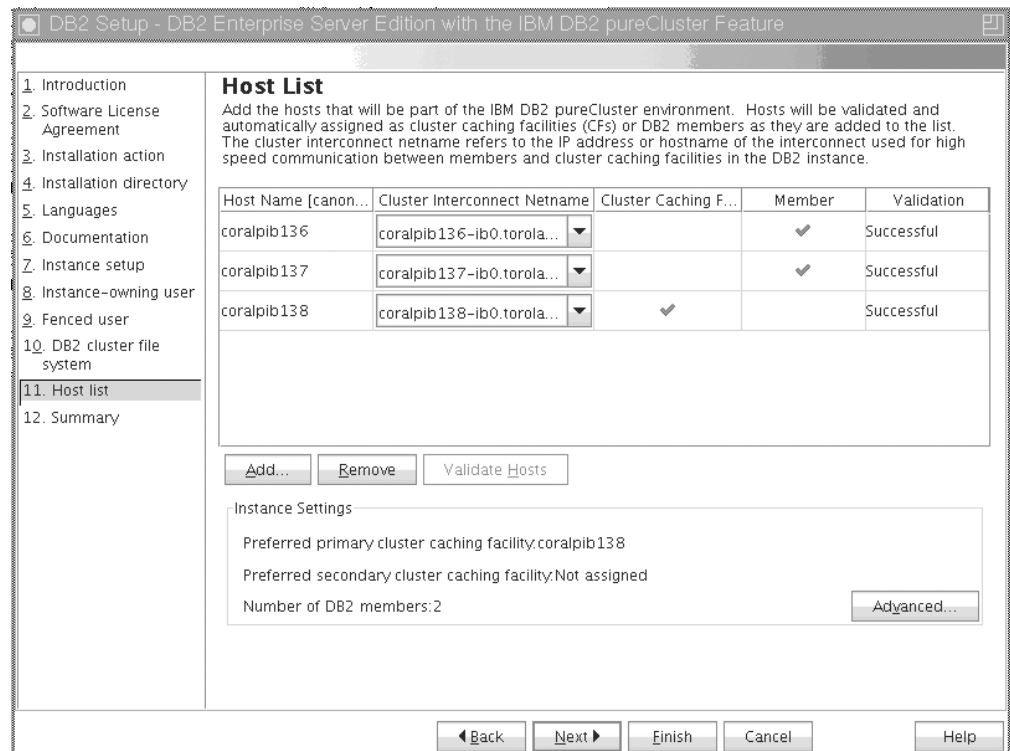
Figure 39. Host List Panel with three hosts (one is the I/H preloaded and two hosts have been added)
