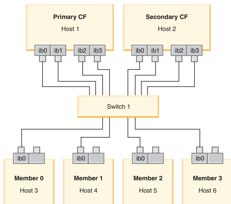
Figure 17. The 2 CFs and four members connect to one switch.
