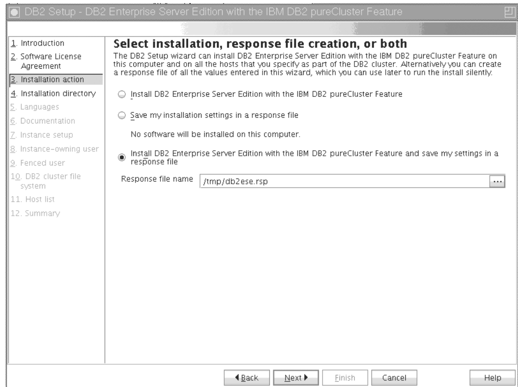
Figure 28. Select installation, response file creation, or both Panel
