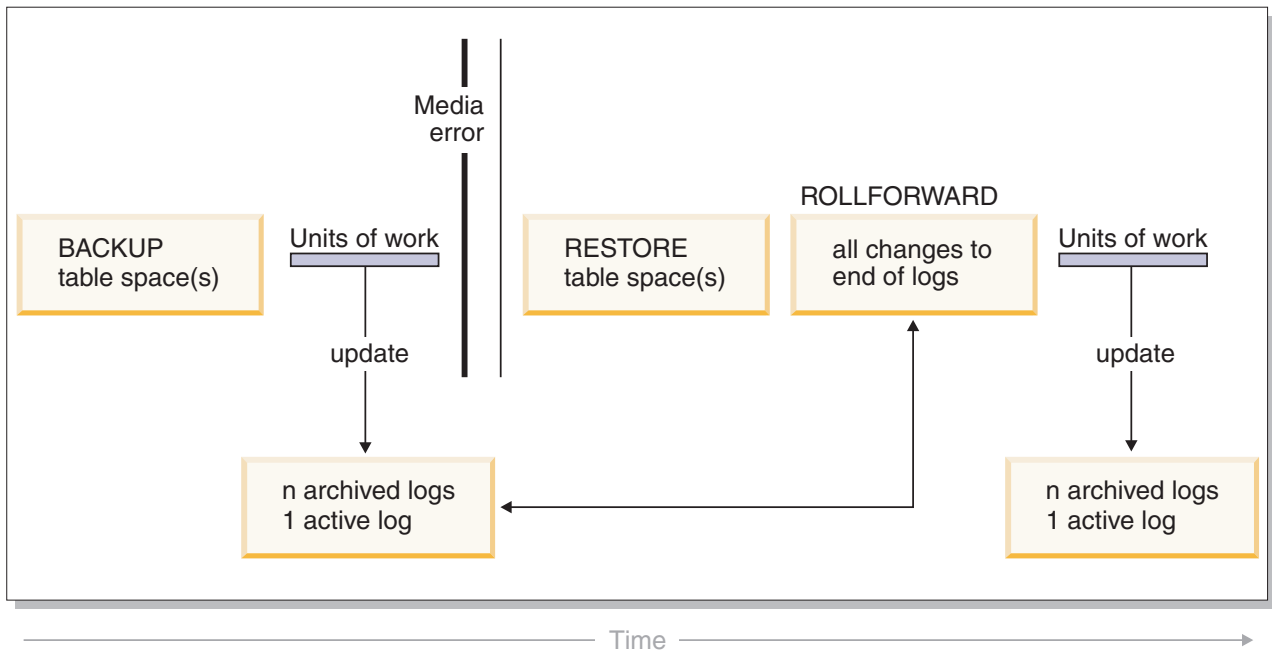
Figure 21. Table Space Rollforward Recovery. There can be more than one active log in the case of a long-running transaction.
