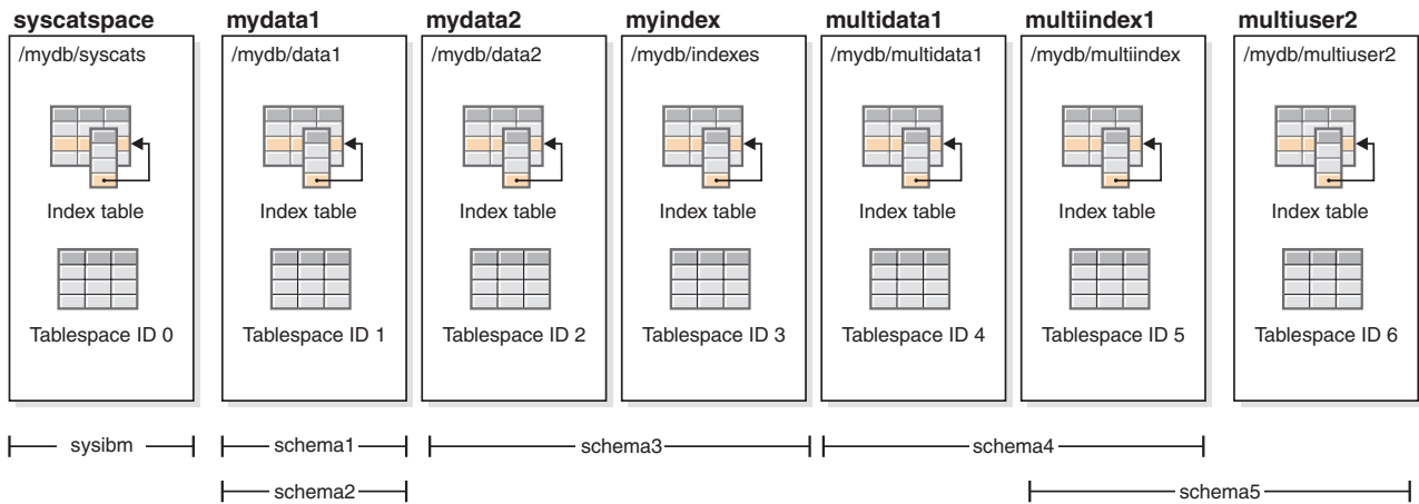
Figure 26. ORIGINALDB database
