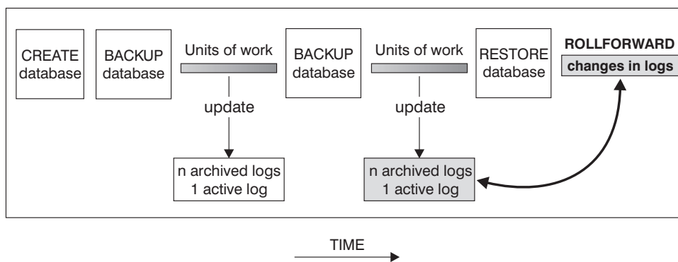
Figure 20. Database Rollforward Recovery. There can be more than one active log in the case of a long-running transaction.
