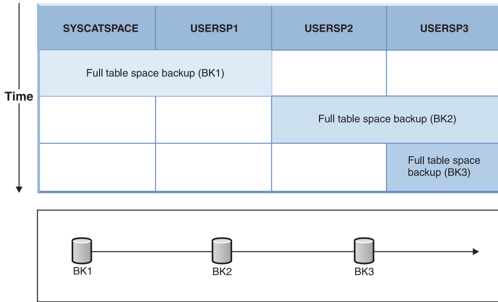
Figure 24. Backup images available for database SAMPLE
