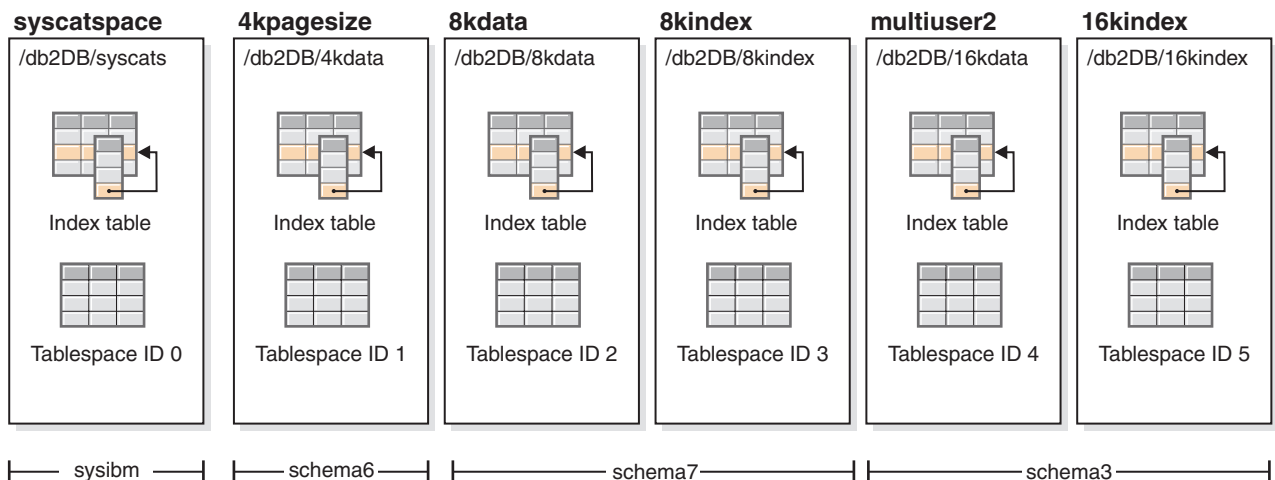
Figure 27. TARGETDB database
