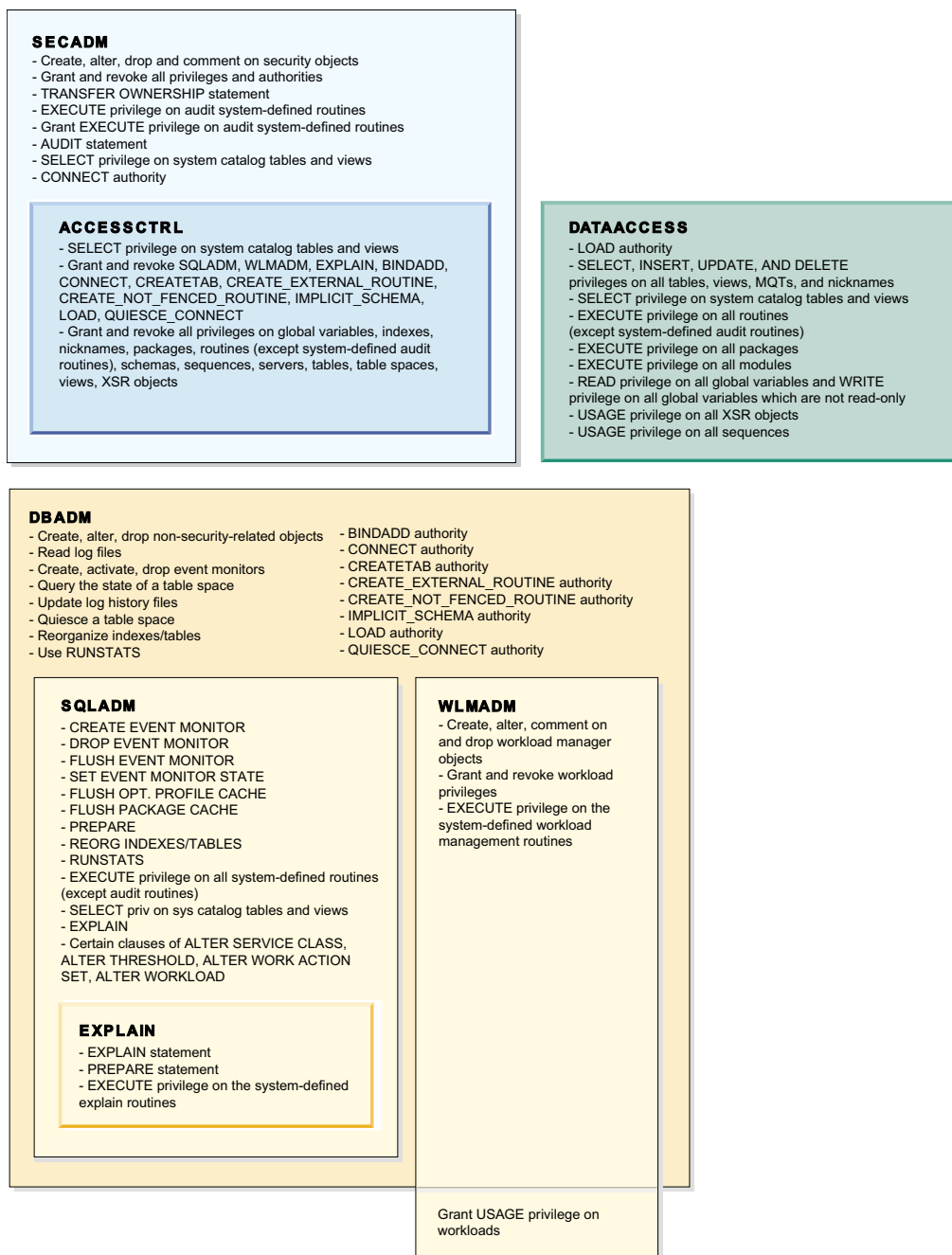
Figure 2. Database-level authorities
