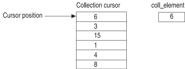
Figure 5-4. Collection Cursor After Fetch First
