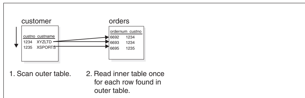
Figure 10-1. Nested-loop join
