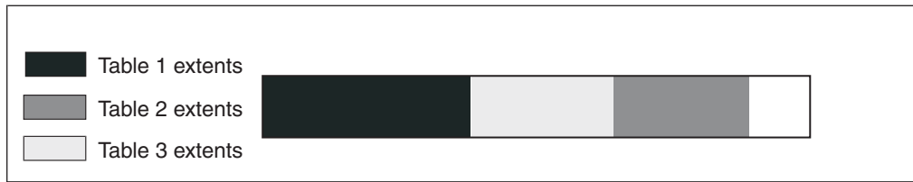
Figure 6-13. A dbspace reorganized to eliminate interleaved extents
