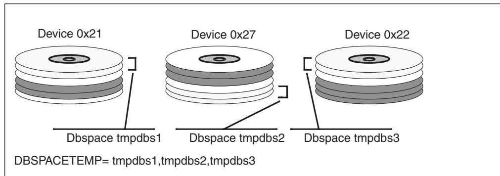
Figure 6-4. Dbspaces for temporary tables and sort files
