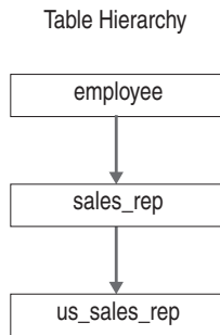
Figure 2-3. Example of Typed Table Hierarchy
