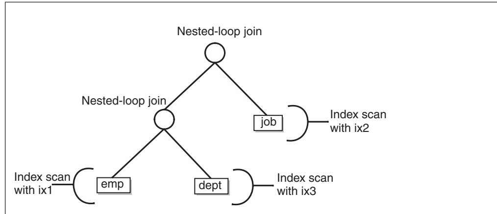
Figure 11-2. Possible query plan without directives
