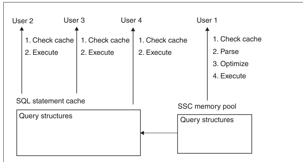
Figure 4-4. Database server actions when using the SQL statement cache
