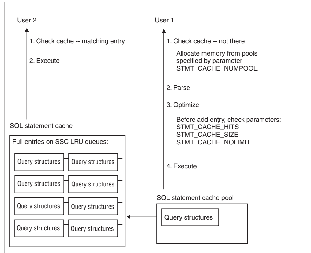
Figure 4-5. Configuration parameters that affect the SQL statement cache
