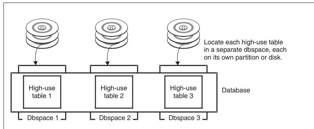
Figure 6-1. Isolating high-use tables
