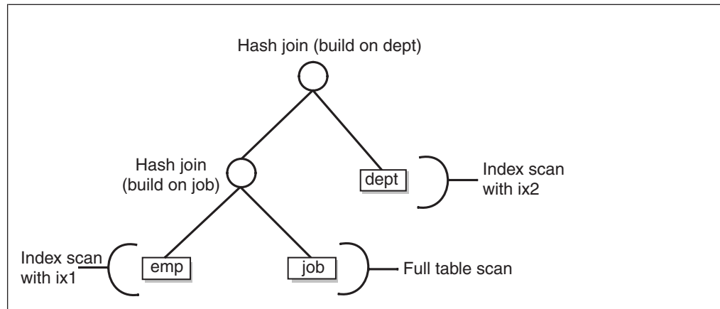
Figure 11-3. Possible query plan with directives
