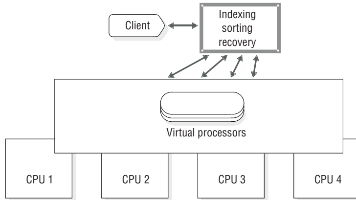
Figure 4-2. Parallel processing
