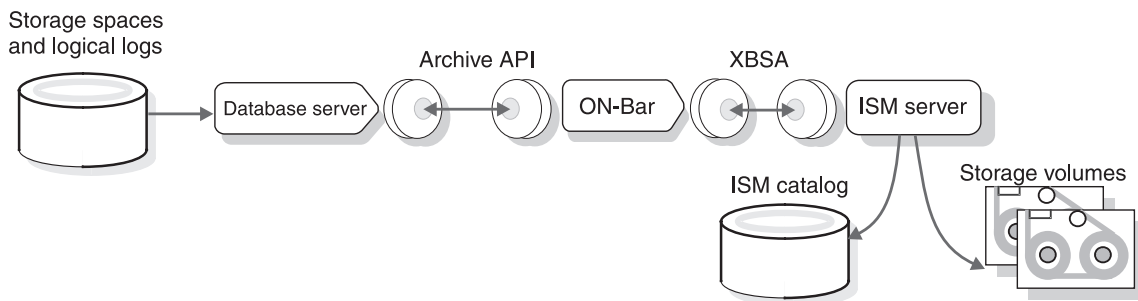
Figure 1-2. Data Movement During an ON-Bar Backup
