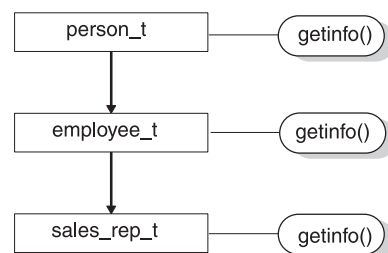
Figure 9-3. Example of routine overloading in a type hierarchy
