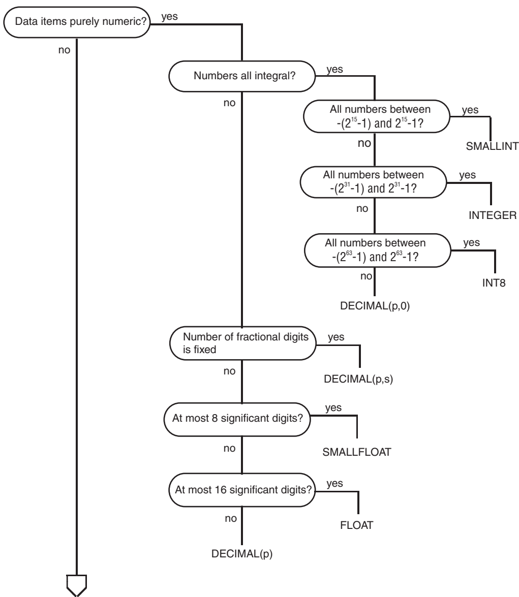
Figure 3-1. Select a data type
