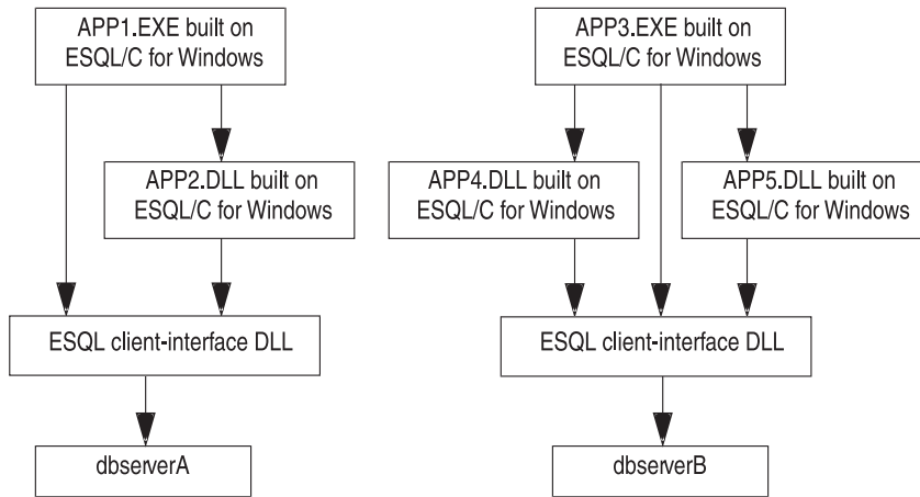
Figure 12-3. Two scenarios in which multiple applications use a single connection to a database server
