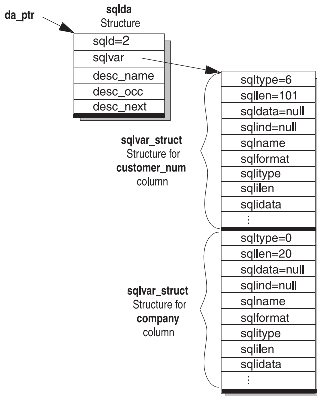
Figure 17-1. Sample sqlda Structure for Two Columns
