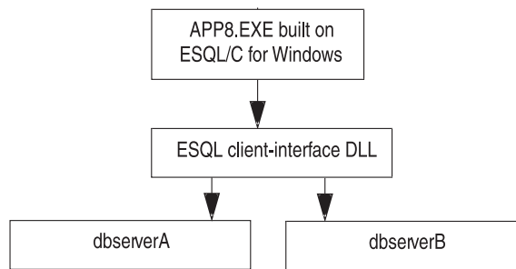
Figure 12-4. One application that uses connections to more than one database server at the same time
