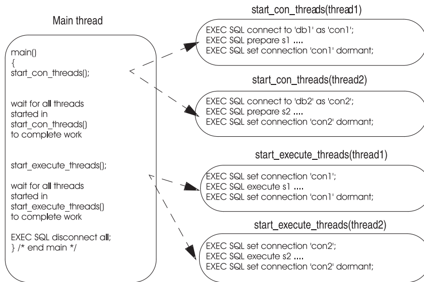
Figure 13-3. Using prepared SQL statements across threads
