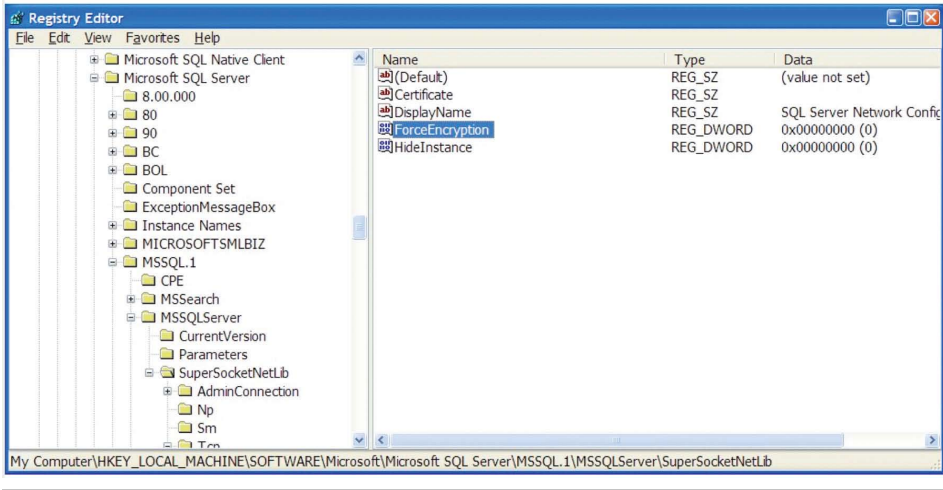
Figure 18: CAS simplifies the process of tracking critical registry values, such as the “Force protocol encryption” registry value for SQL Server.
