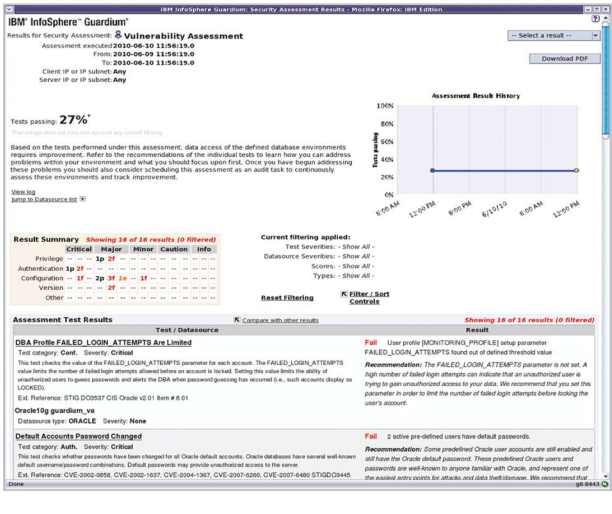
Figure 6: InfoSphere Guardium's Database Vulnerability Assessment module produces summary results that provide an understanding of your overall security posture, along with detailed drill-downs containing concrete recommendations for improvement.
