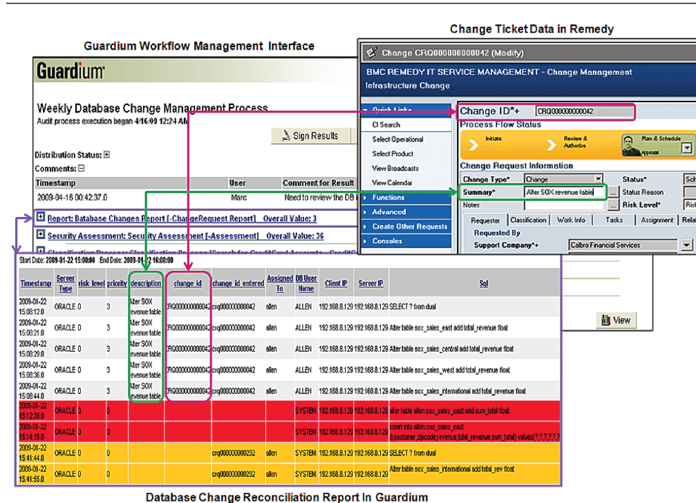
Figure 30: The Enterprise Integrator can be used to import change management information from custom or commercial systems like BMC's Remedy or HP's Peregrine. In this example the Change ID and Summary description are included in a weekly Database Change Report which is distributed and managed using InfoSphere Guardium's workflow capabilities. The report has been structured so actual changes made with no tickets are highlighted in red. Changes in yellow indicate an invalid change number was entered for the change. Displaying the Remedy Summary of the authorized change along with the actual SQL commands executed allows report recipients to verify that changes made correspond to those authorized.
