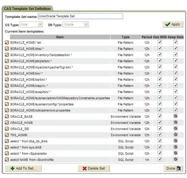
Figure 19: CAS allows you to define the polling period for tracking changes; whether MD5 checksums are used to track changes (rather than timestamps); and whether CAS should also “keep data” to track “before” values.
